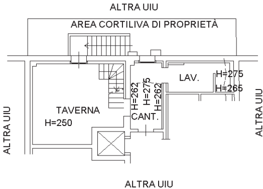
PIANO TERRA
